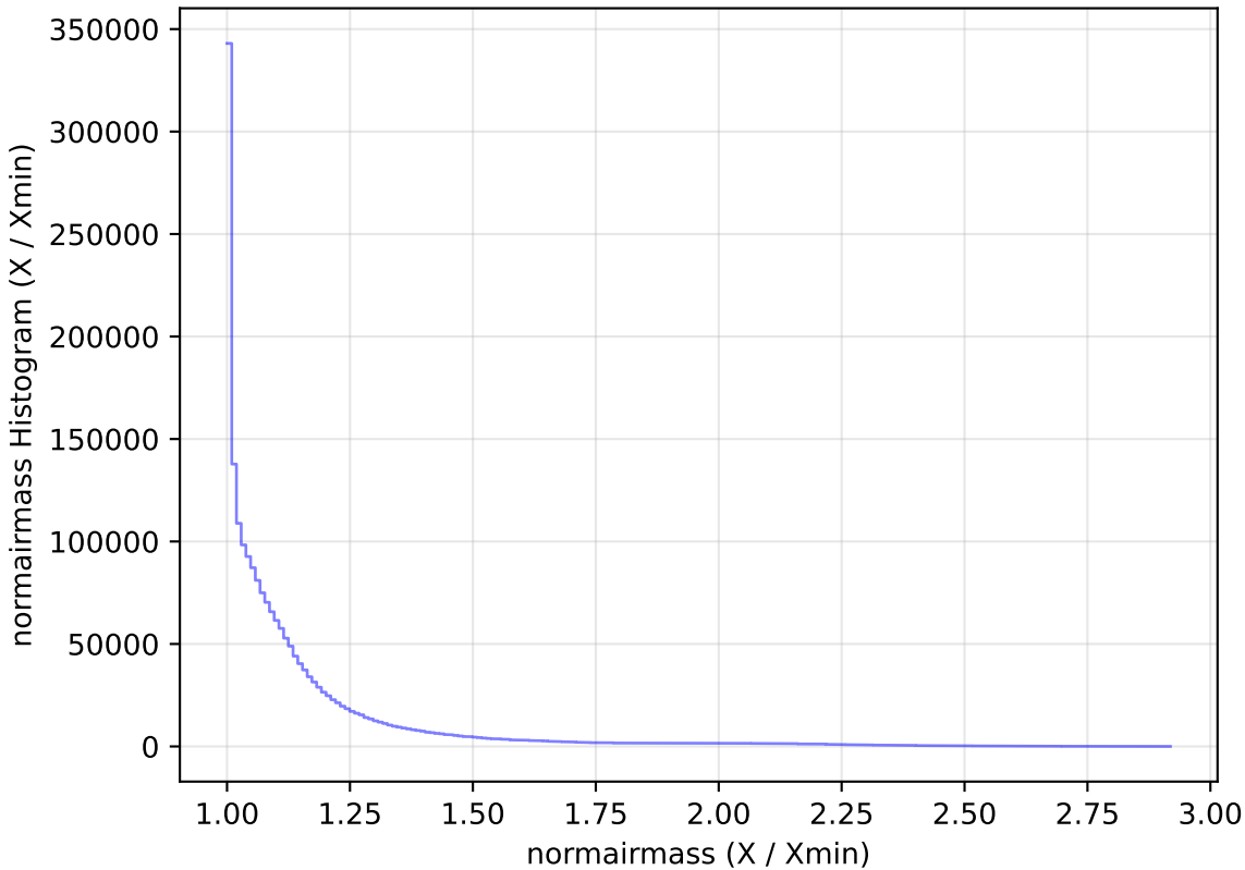
ddf_loaded_half_fl2_v3.4_10yrs All sky all bands: normairmass Histogram
