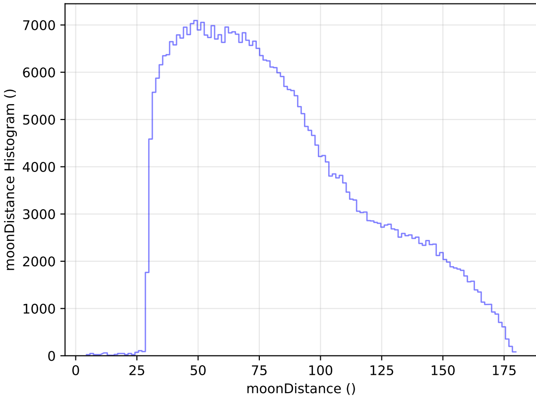
ddf_loaded_half_fl2_v3.4_10yrs WFD z band: moonDistance Histogram
