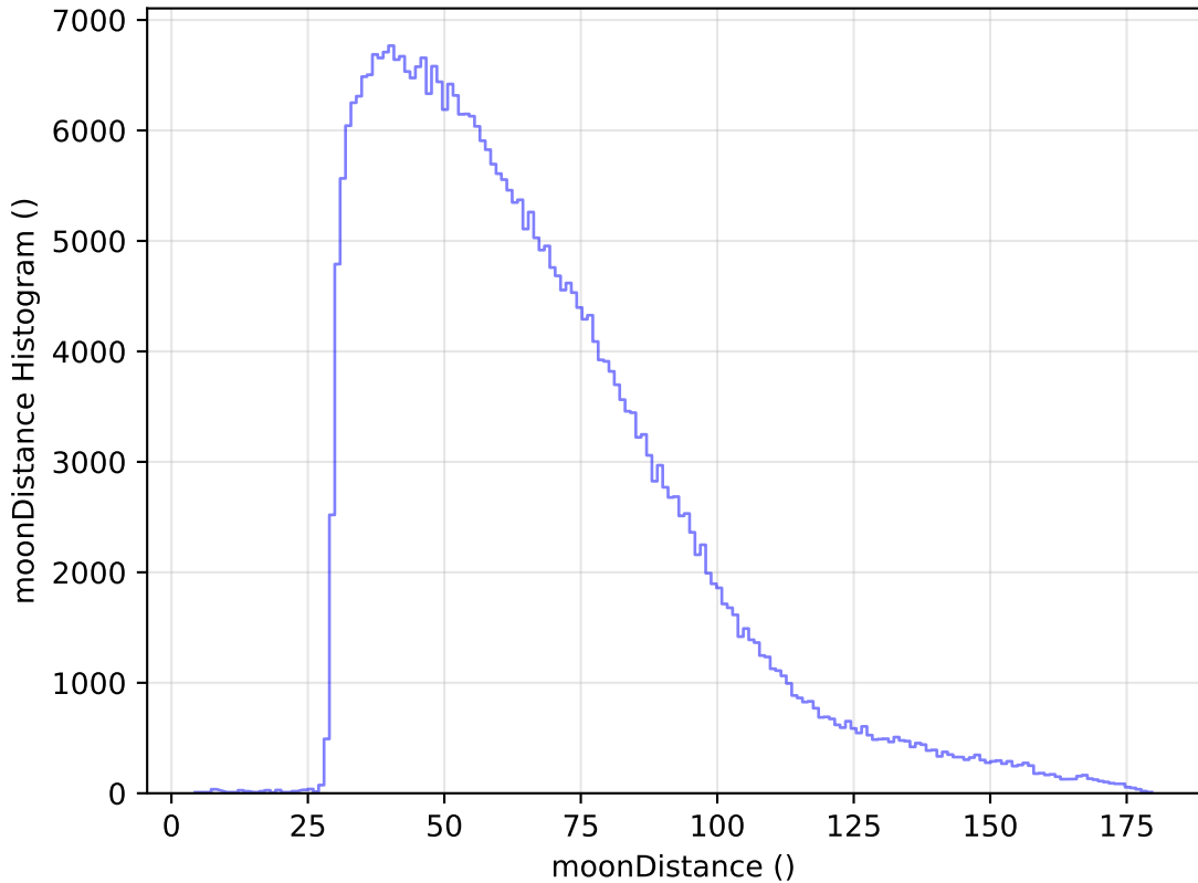
ddf_loaded_half_fl2_v3.4_10yrs WFD y band: moonDistance Histogram
