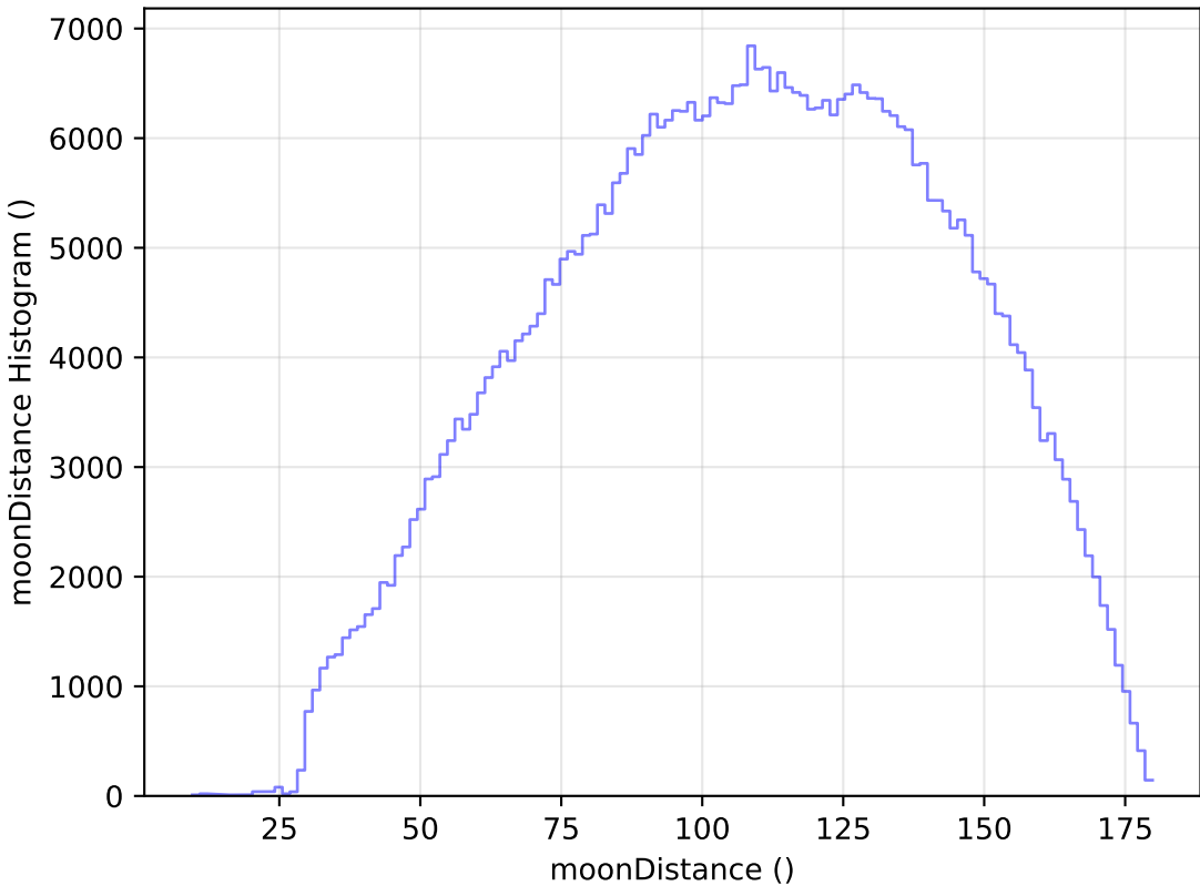
ddf_loaded_half_fl2_v3.4_10yrs WFD r band: moonDistance Histogram
