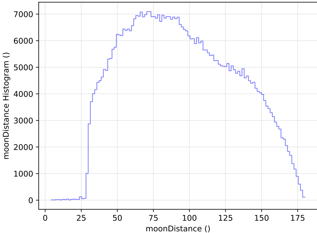
ddf_loaded_half_fl2_v3.4_10yrs WFD i band: moonDistance Histogram
