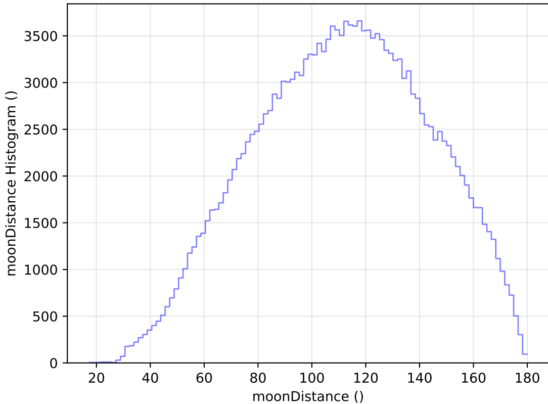
ddf_loaded_half_fl2_v3.4_10yrs WFD g band: moonDistance Histogram
