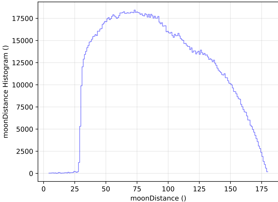
ddf_loaded_half_fl2_v3.4_10yrs WFD all bands: moonDistance Histogram
