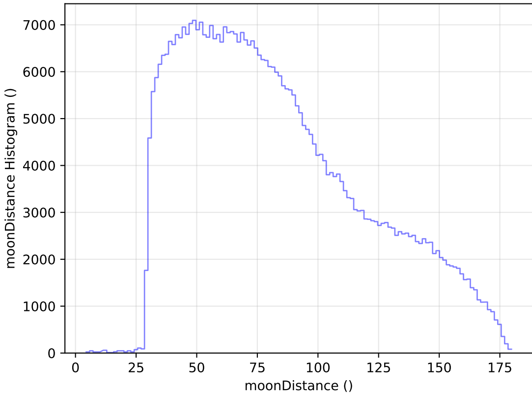
ddf_loaded_half_fl2_v3.4_10yrs All sky z band: moonDistance Histogram
