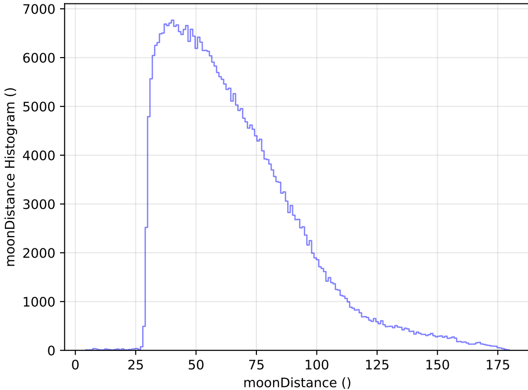
ddf_loaded_half_fl2_v3.4_10yrs All sky y band: moonDistance Histogram
