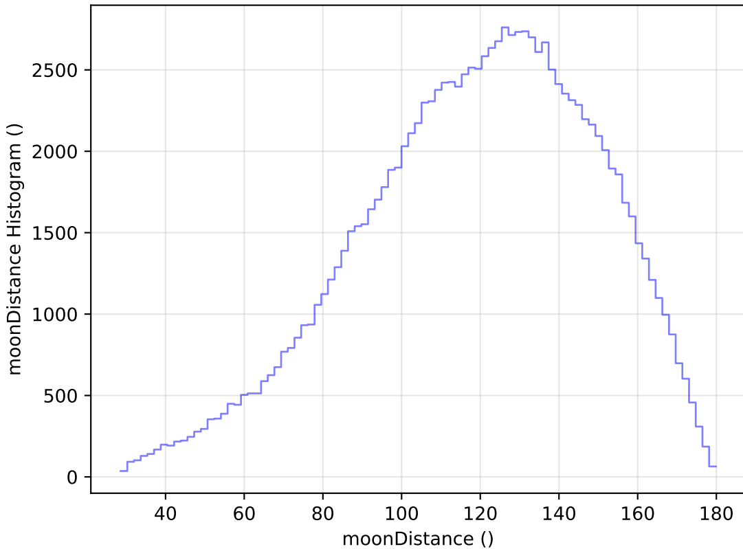
ddf_loaded_half_fl2_v3.4_10yrs All sky u band: moonDistance Histogram
