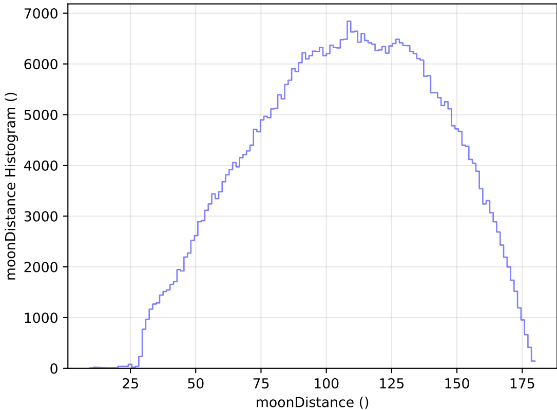
ddf_loaded_half_fl2_v3.4_10yrs All sky r band: moonDistance Histogram
