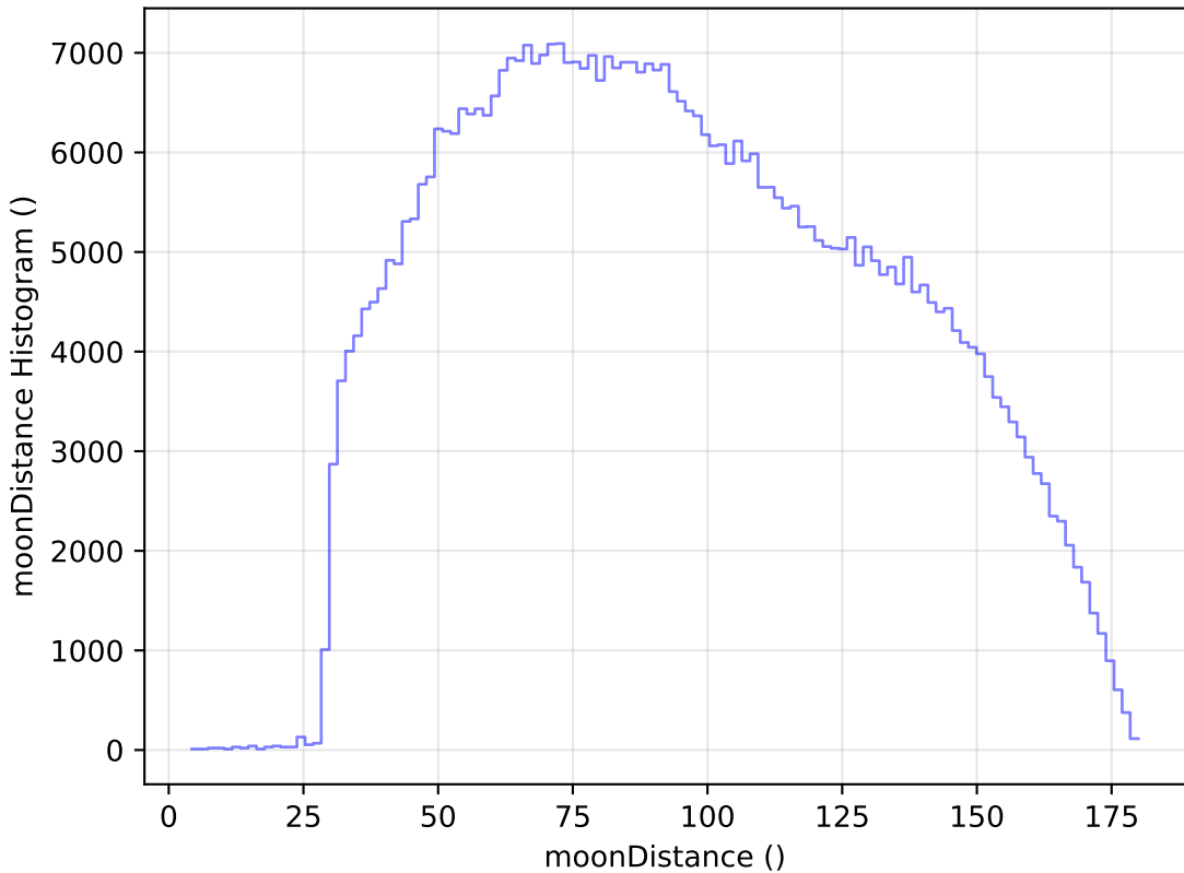
ddf_loaded_half_fl2_v3.4_10yrs All sky i band: moonDistance Histogram
