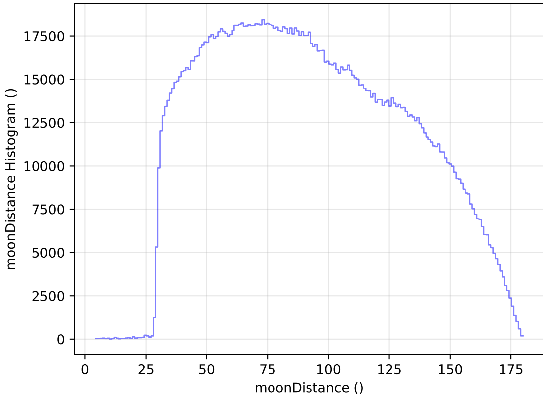
ddf_loaded_half_fl2_v3.4_10yrs All sky all bands: moonDistance Histogram
