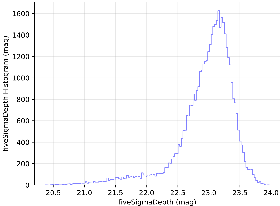
ddf_loaded_half_fl2_v3.4_10yrs Yr 1 z band: fiveSigmaDepth Histogram
