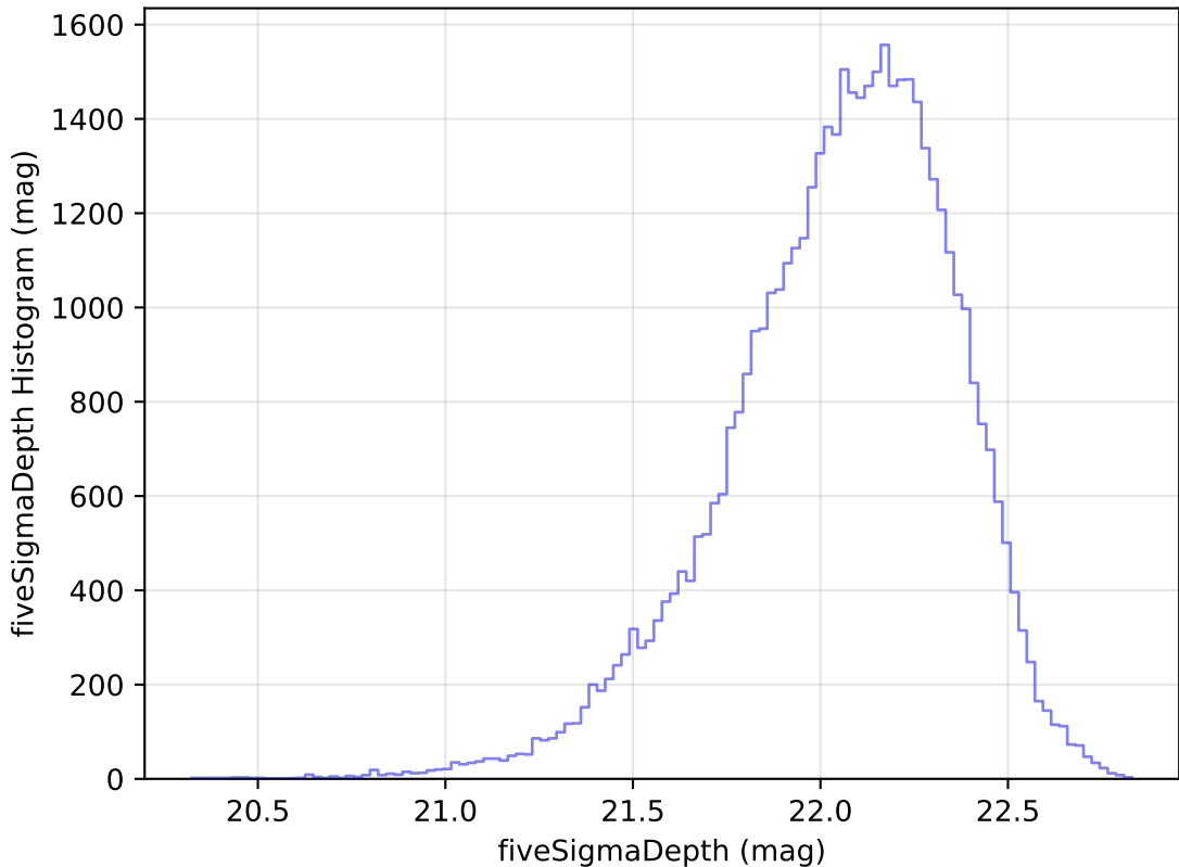
ddf_loaded_half_fl2_v3.4_10yrs Yr 1 y band: fiveSigmaDepth Histogram
