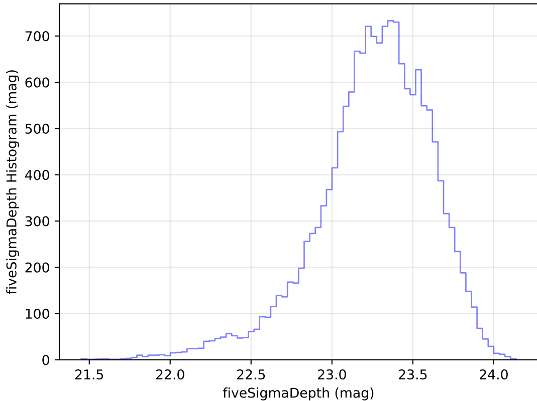
ddf_loaded_half_fl2_v3.4_10yrs Yr 1 u band: fiveSigmaDepth Histogram
