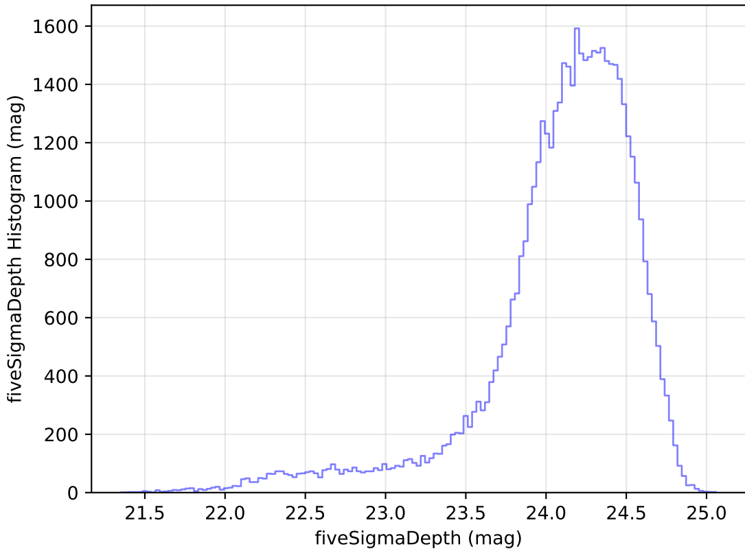
ddf_loaded_half_fl2_v3.4_10yrs Yr 1 r band: fiveSigmaDepth Histogram
