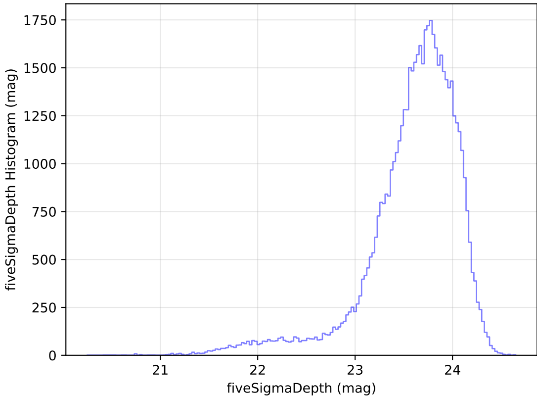
ddf_loaded_half_fl2_v3.4_10yrs Yr 1 i band: fiveSigmaDepth Histogram
