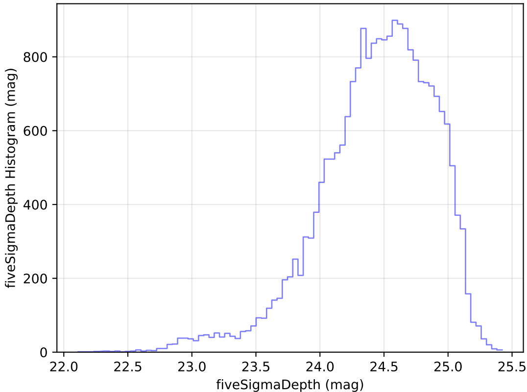
ddf_loaded_half_fl2_v3.4_10yrs Yr 1 g band: fiveSigmaDepth Histogram
