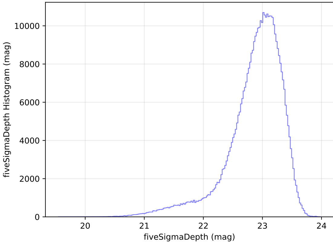
ddf_loaded_half_fl2_v3.4_10yrs WFD z band: fiveSigmaDepth Histogram
