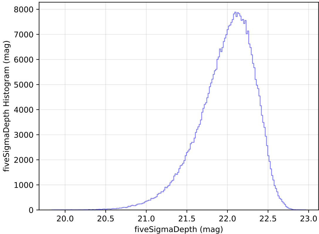
ddf_loaded_half_fl2_v3.4_10yrs WFD y band: fiveSigmaDepth Histogram
