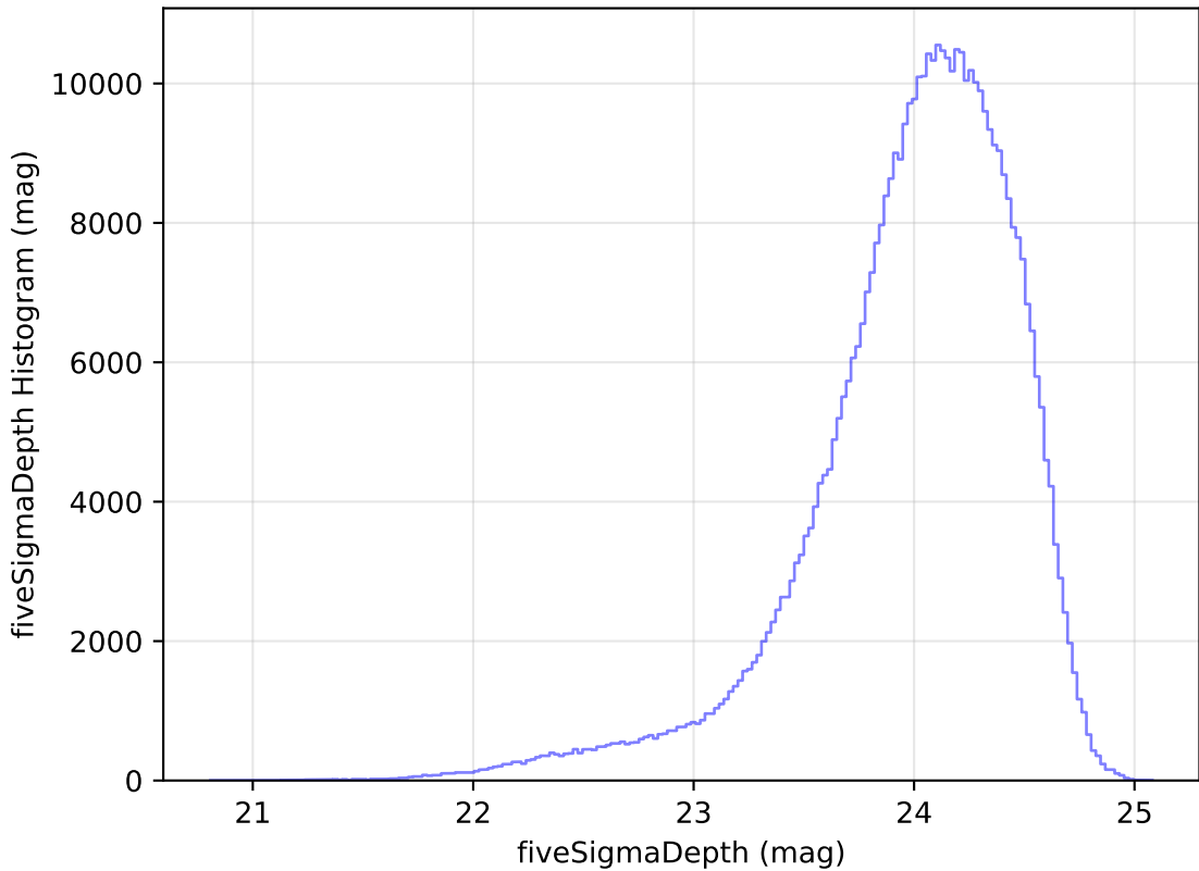
ddf_loaded_half_fl2_v3.4_10yrs WFD r band: fiveSigmaDepth Histogram
