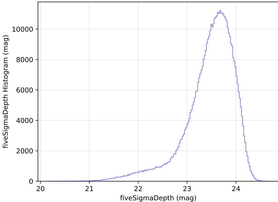
ddf_loaded_half_fl2_v3.4_10yrs WFD i band: fiveSigmaDepth Histogram
