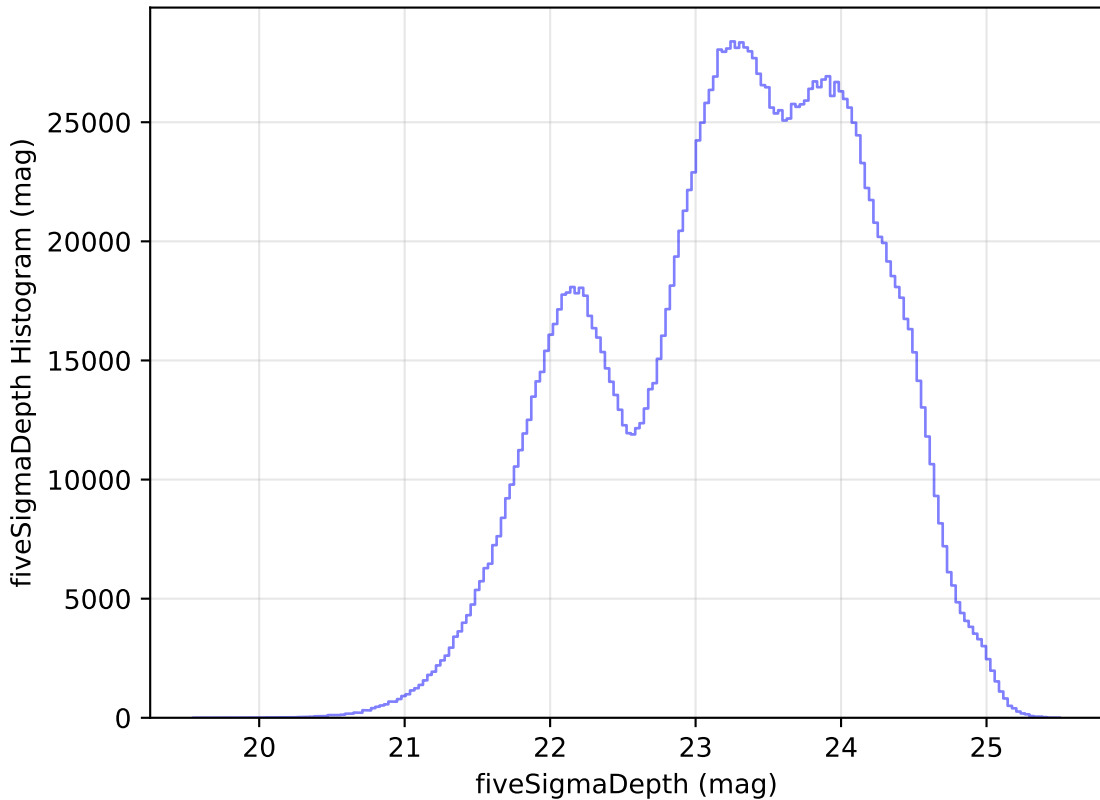
ddf_loaded_half_fl2_v3.4_10yrs WFD all bands: fiveSigmaDepth Histogram
