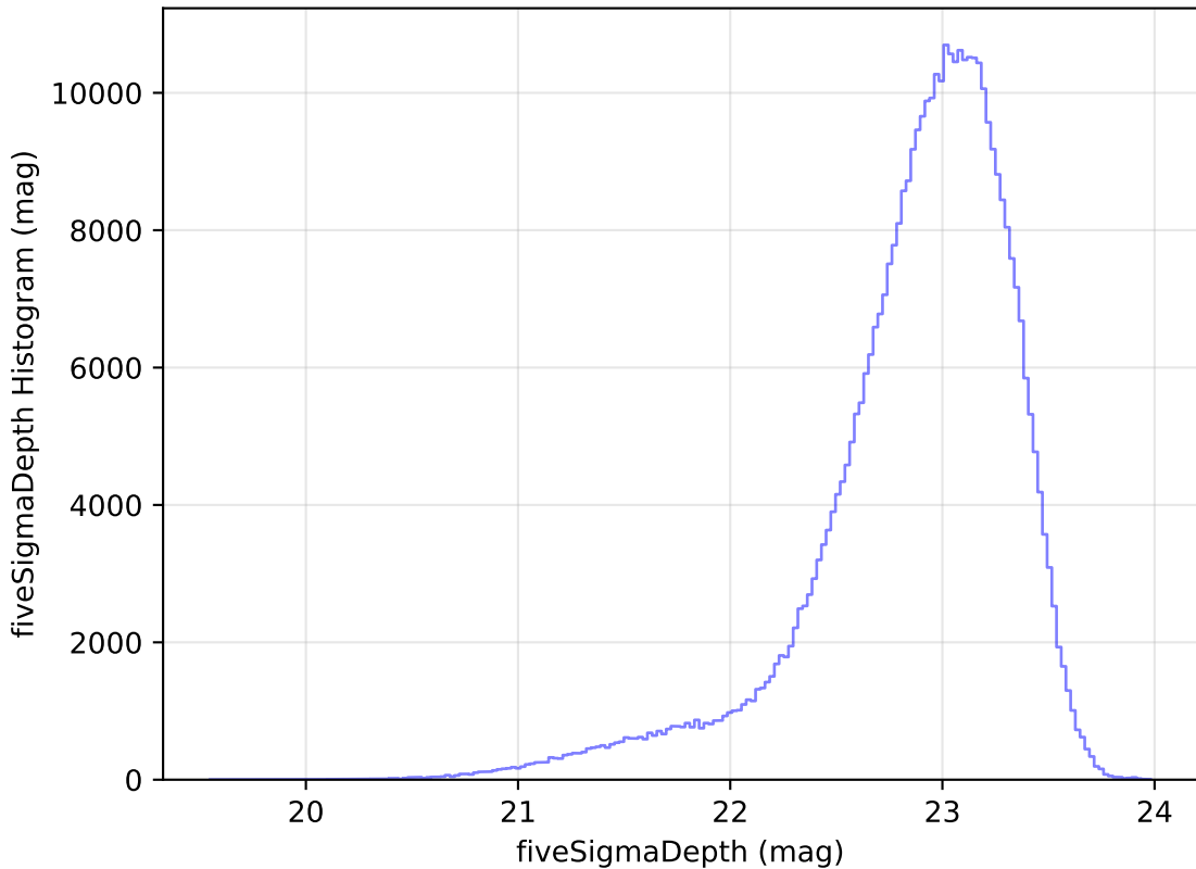
ddf_loaded_half_fl2_v3.4_10yrs All sky z band: fiveSigmaDepth Histogram
