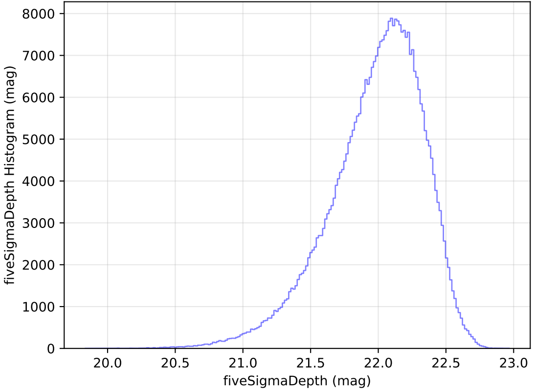
ddf_loaded_half_fl2_v3.4_10yrs All sky y band: fiveSigmaDepth Histogram
