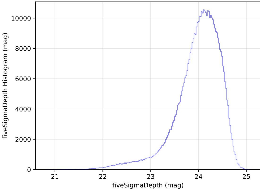
ddf_loaded_half_fl2_v3.4_10yrs All sky r band: fiveSigmaDepth Histogram
