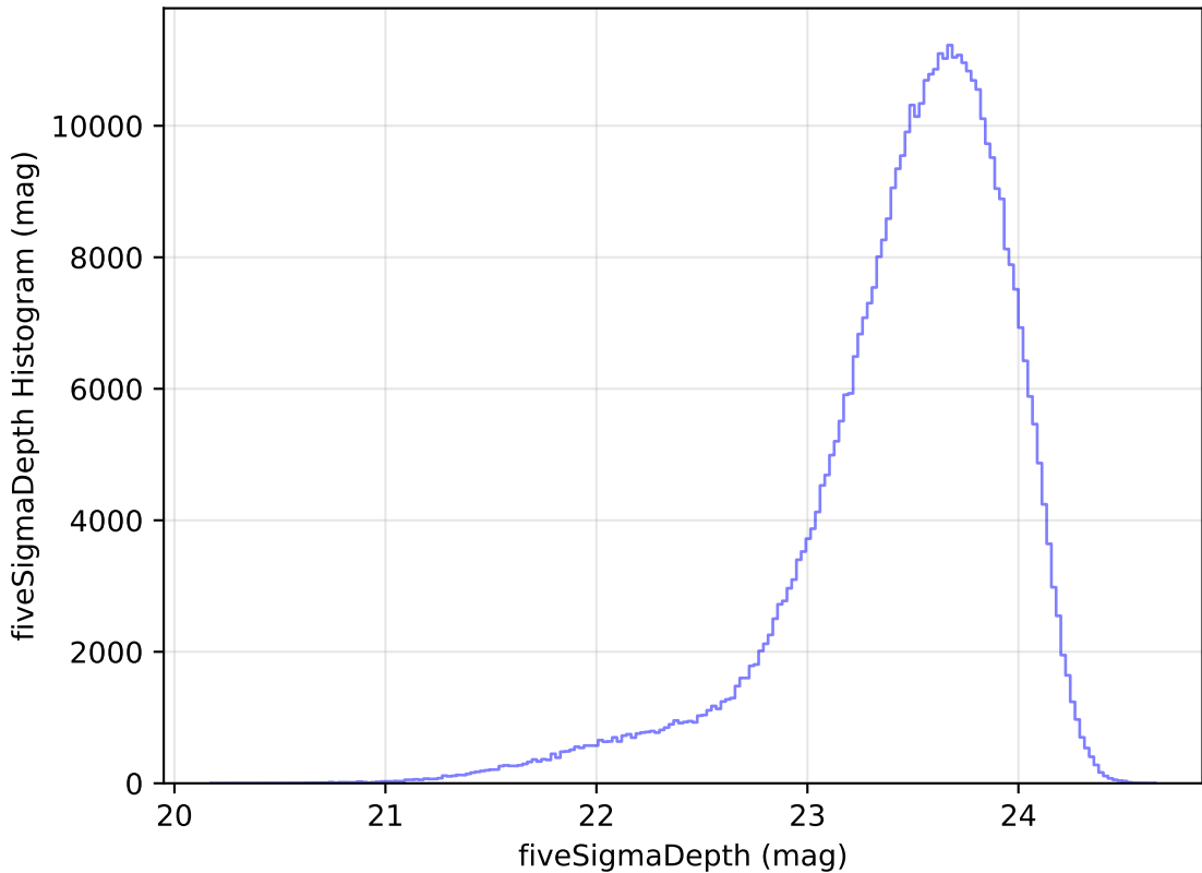
ddf_loaded_half_fl2_v3.4_10yrs All sky i band: fiveSigmaDepth Histogram
