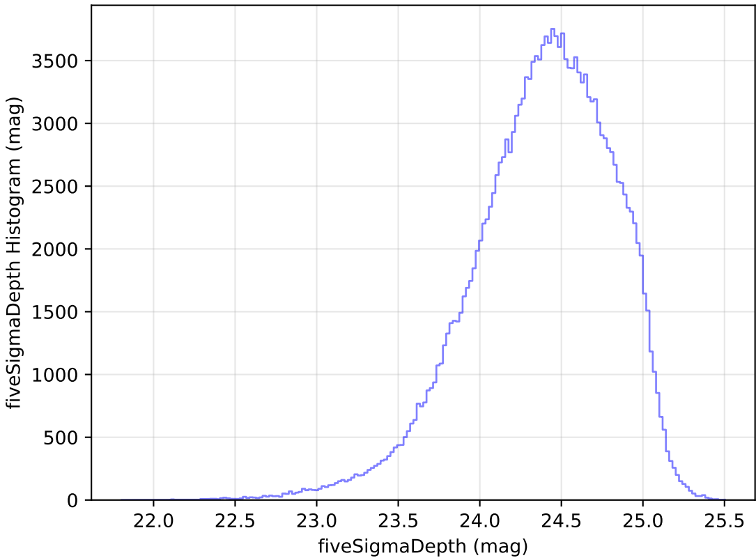
ddf_loaded_half_fl2_v3.4_10yrs All sky g band: fiveSigmaDepth Histogram
