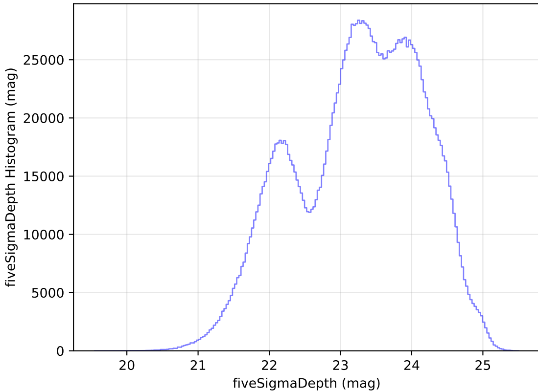
ddf_loaded_half_fl2_v3.4_10yrs All sky all bands: fiveSigmaDepth Histogram
