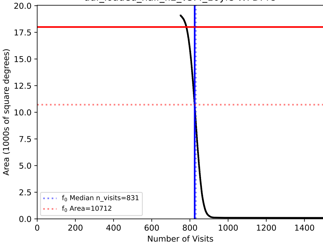
ddf_loaded_half_fl2_v3.4_10yrs WFD: fO
