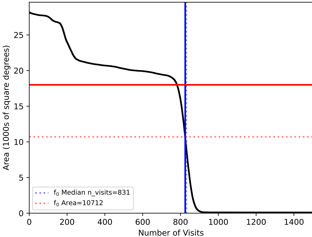
ddf_loaded_half_fl2_v3.4_10yrs All sky: fO
