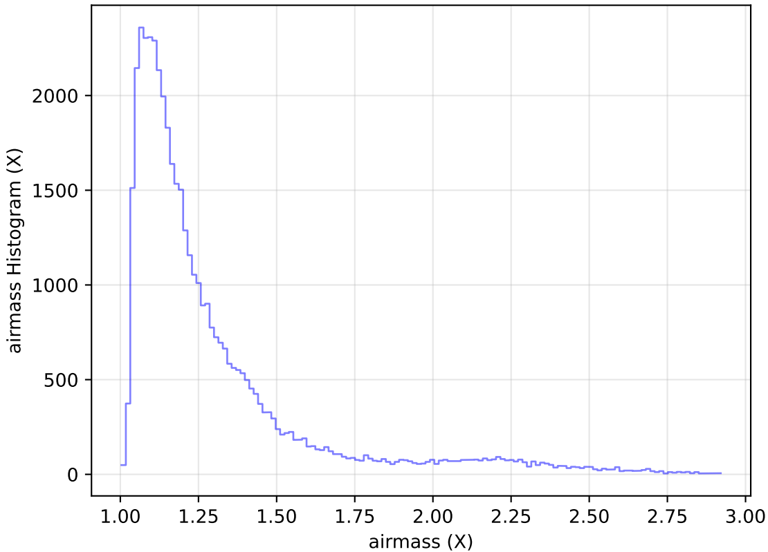
ddf_loaded_half_fl2_v3.4_10yrs Yr 1 z band: airmass Histogram
