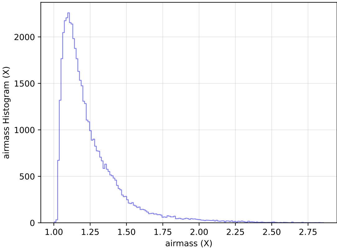
ddf_loaded_half_fl2_v3.4_10yrs Yr 1 y band: airmass Histogram
