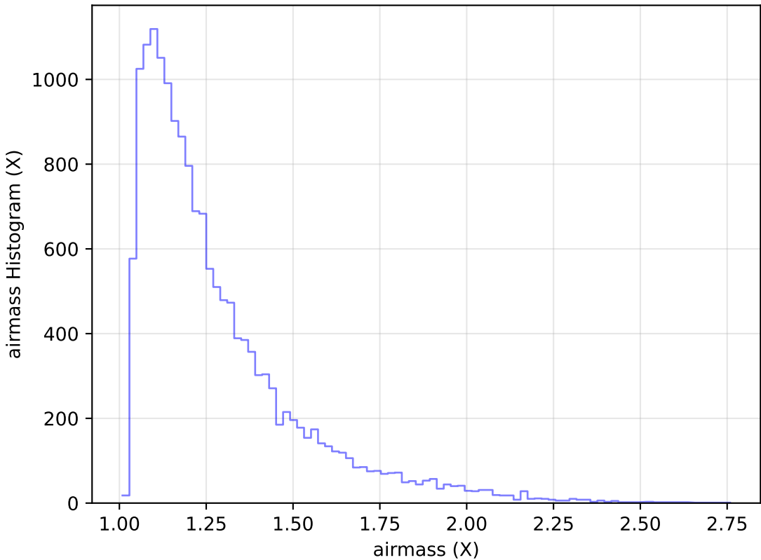
ddf_loaded_half_fl2_v3.4_10yrs Yr 1 u band: airmass Histogram
