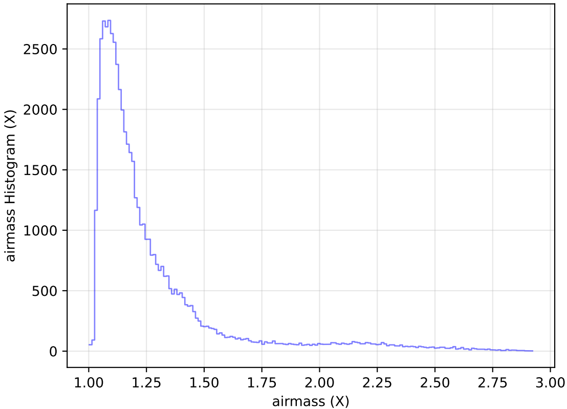
ddf_loaded_half_fl2_v3.4_10yrs Yr 1 i band: airmass Histogram
