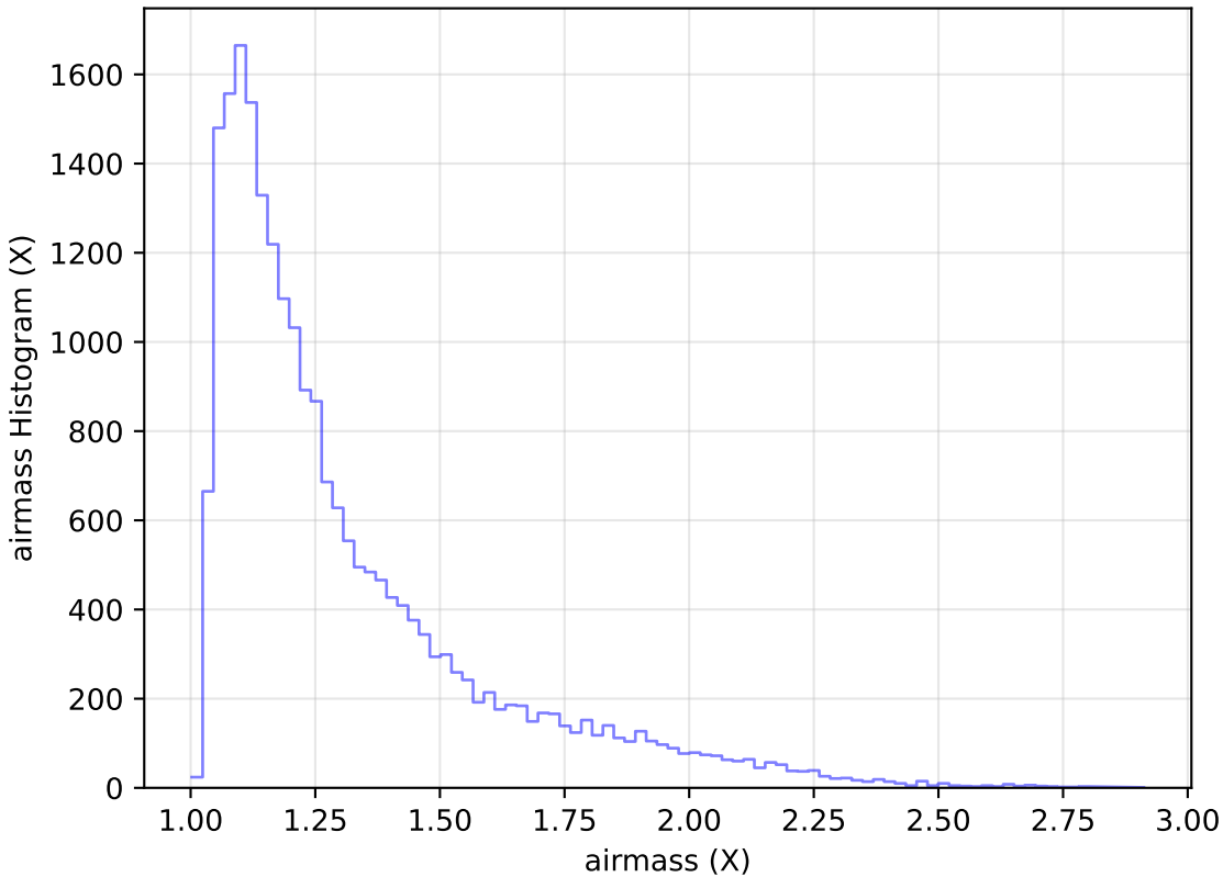
ddf_loaded_half_fl2_v3.4_10yrs Yr 1 g band: airmass Histogram
