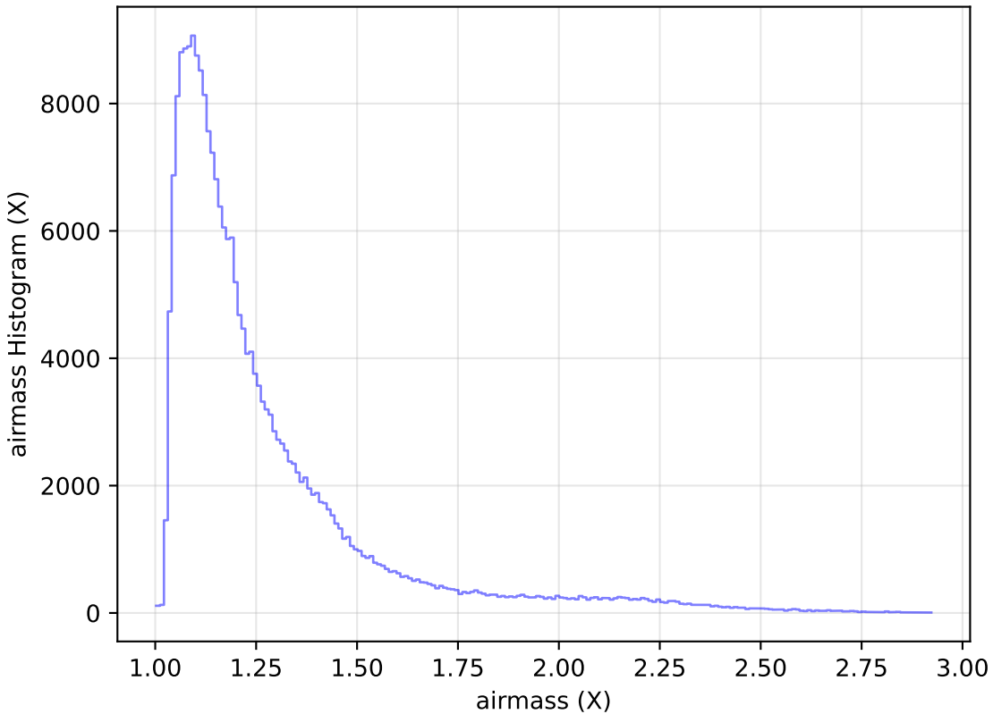
ddf_loaded_half_fl2_v3.4_10yrs Yr 1 all bands: airmass Histogram
