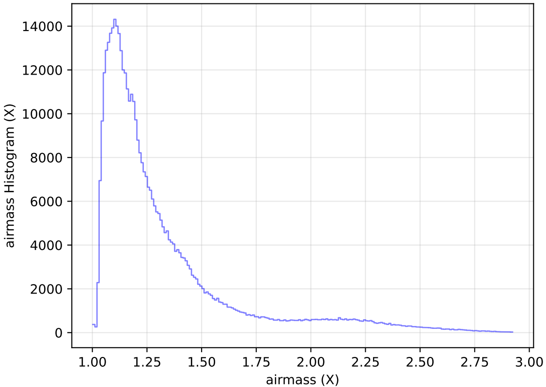
ddf_loaded_half_fl2_v3.4_10yrs WFD z band: airmass Histogram
