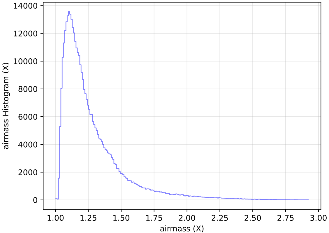
ddf_loaded_half_fl2_v3.4_10yrs WFD y band: airmass Histogram
