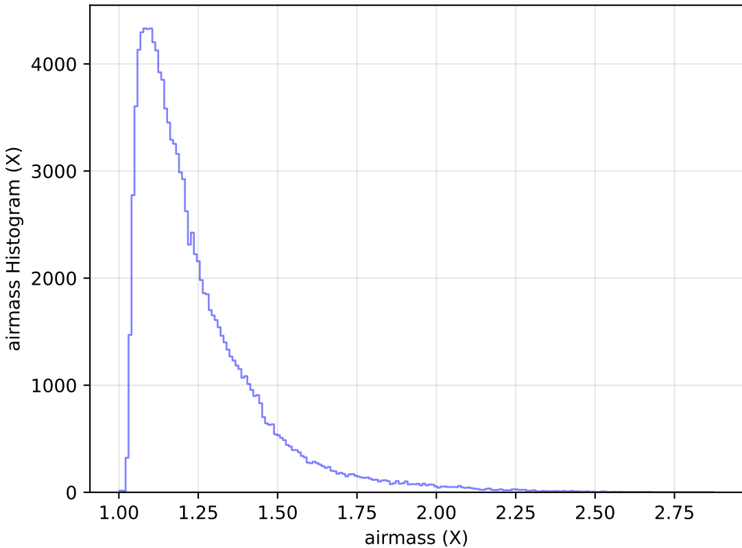
ddf_loaded_half_fl2_v3.4_10yrs WFD u band: airmass Histogram
