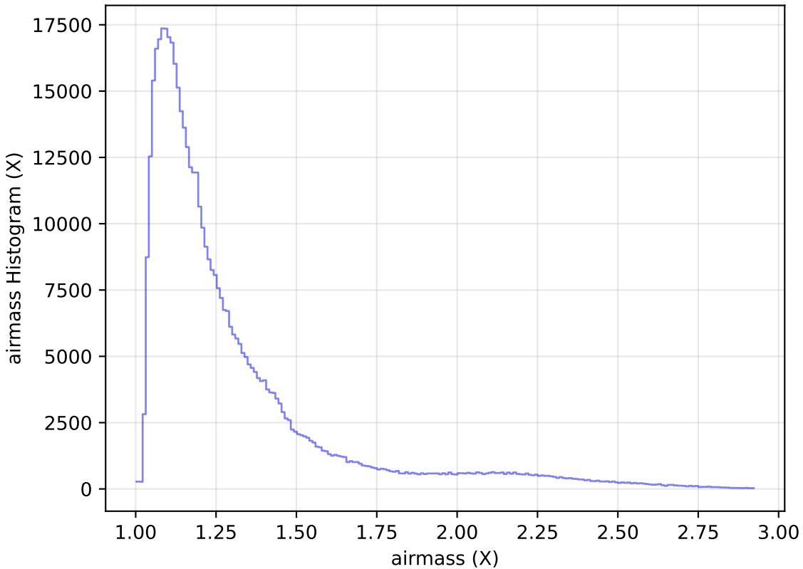
ddf_loaded_half_fl2_v3.4_10yrs WFD i band: airmass Histogram
