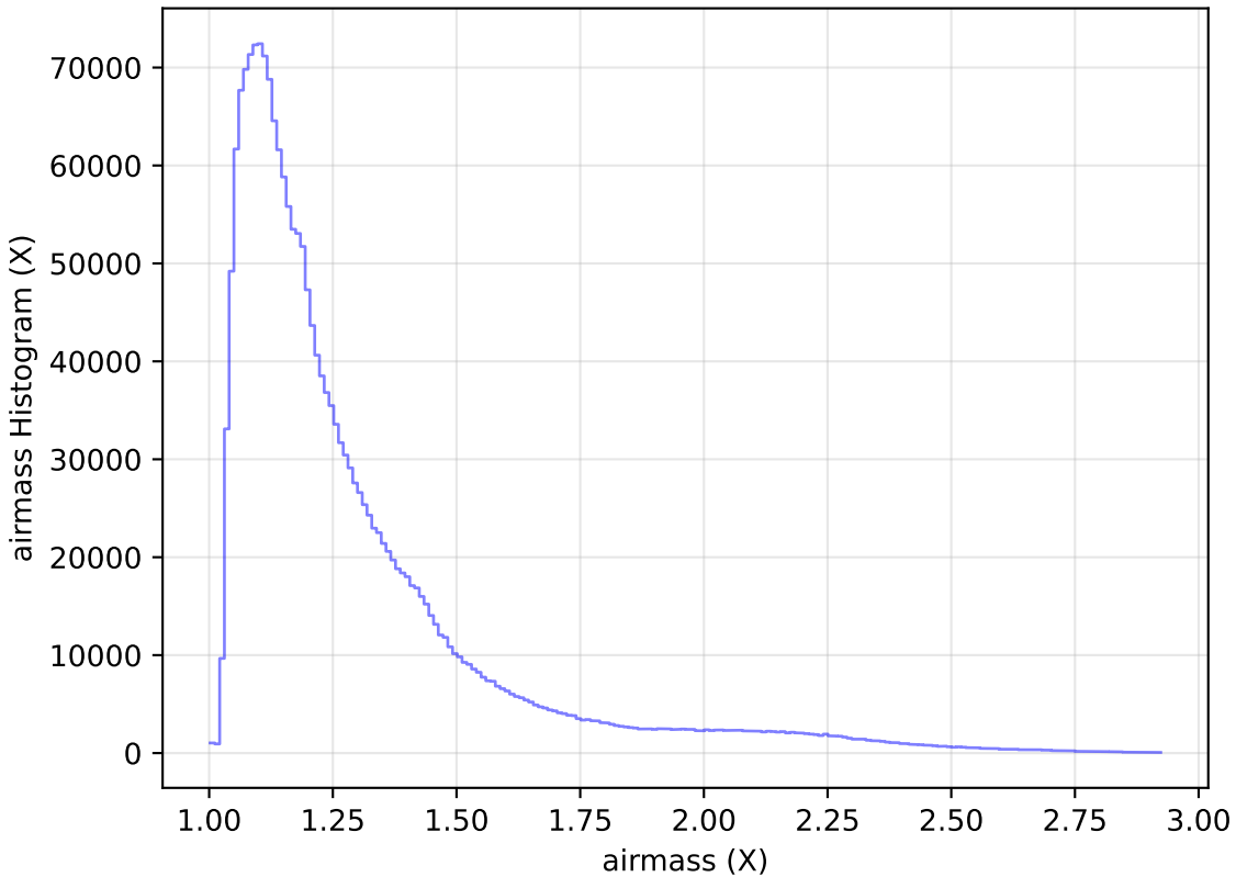
ddf_loaded_half_fl2_v3.4_10yrs WFD all bands: airmass Histogram
