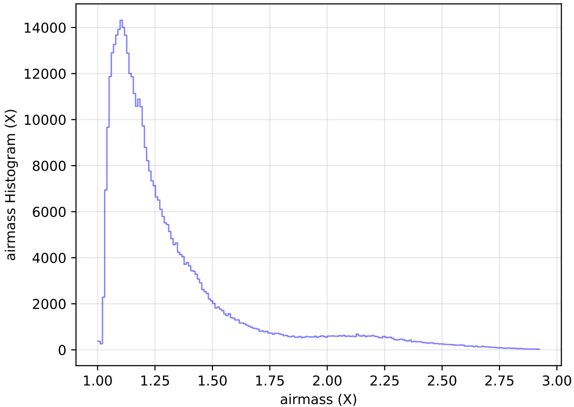
ddf_loaded_half_fl2_v3.4_10yrs All sky z band: airmass Histogram
