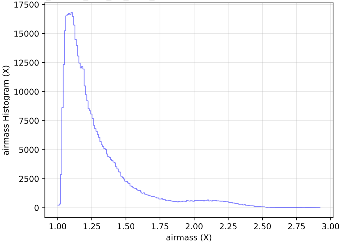
ddf_loaded_half_fl2_v3.4_10yrs All sky r band: airmass Histogram
