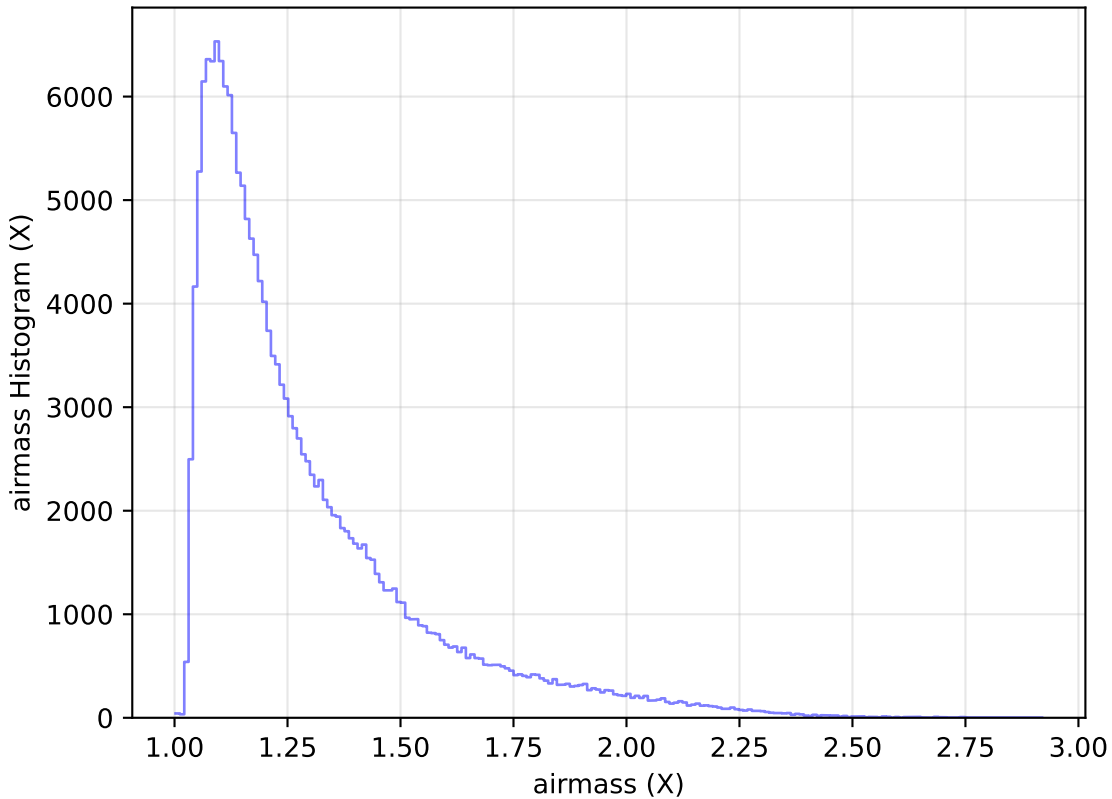
ddf_loaded_half_fl2_v3.4_10yrs All sky g band: airmass Histogram
