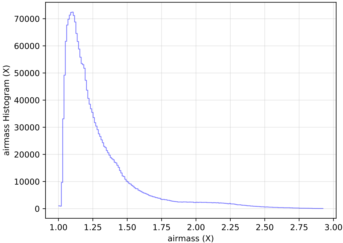
ddf_loaded_half_fl2_v3.4_10yrs All sky all bands: airmass Histogram
