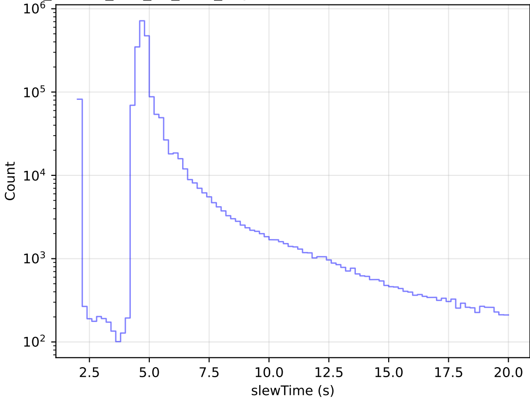
ddf_loaded_half_fl2_v3.4_10yrs All visits: Zoom Slew Time Histogram
