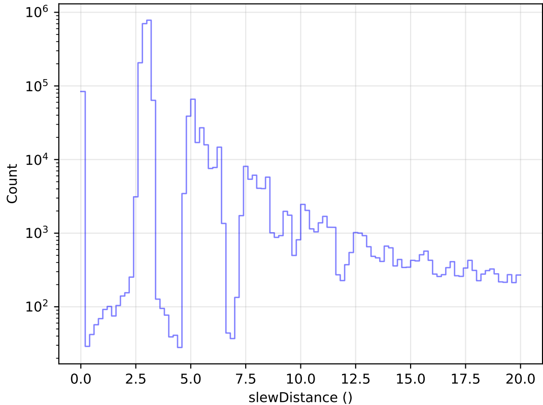
ddf_loaded_half_fl2_v3.4_10yrs All visits: Zoom Slew Distance Histogram
