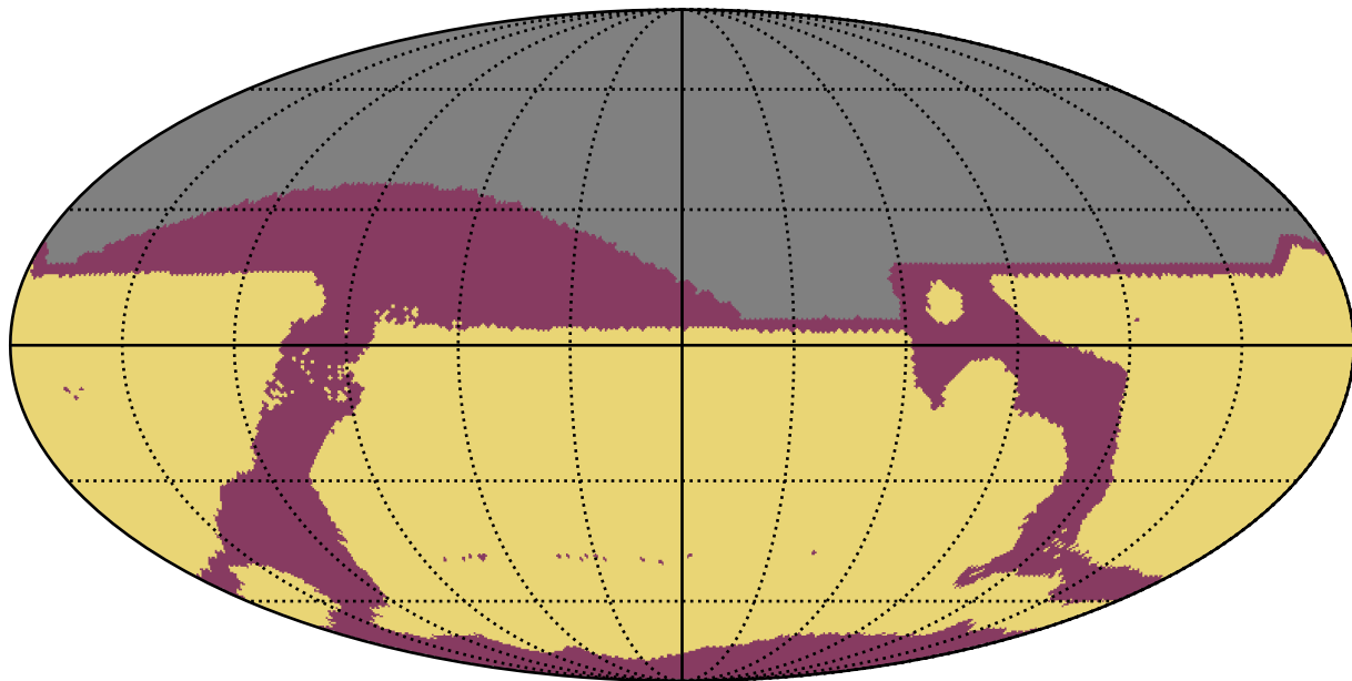
ddf_loaded_half_fl2_v3.4_10yrs All sky: RapidRevisits
